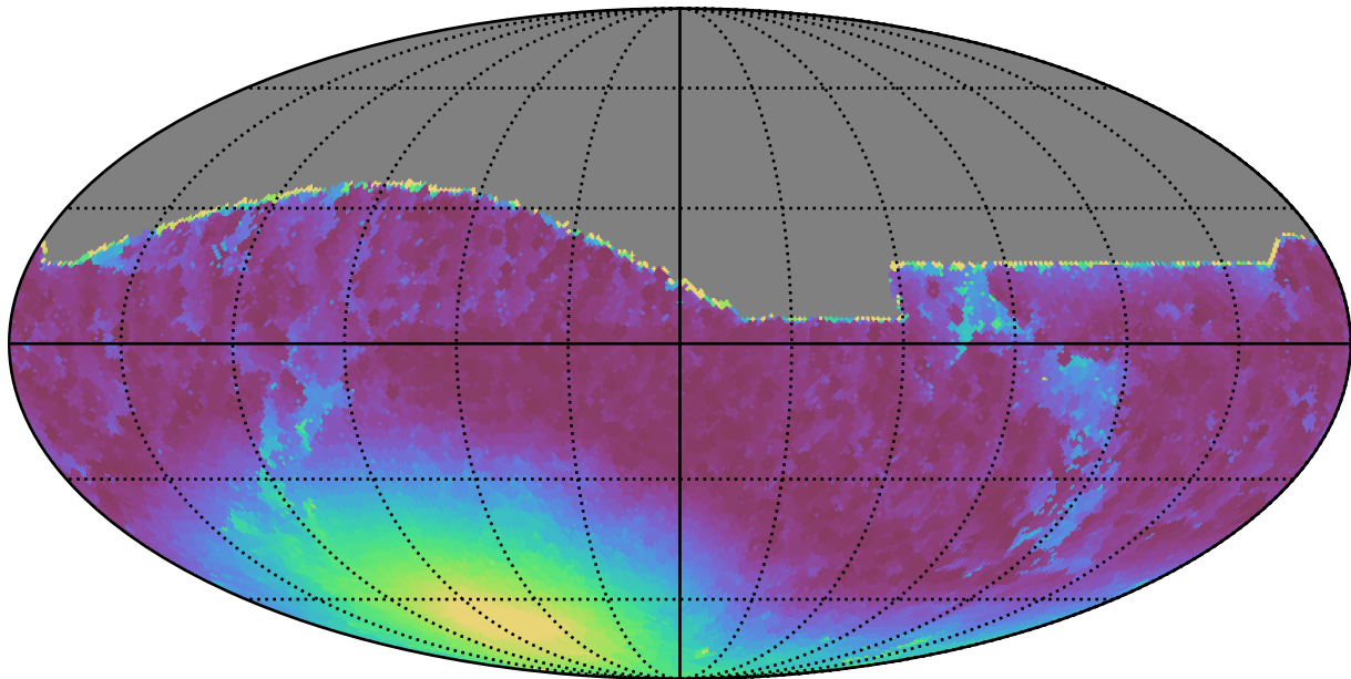
weather_cloudso20v3.4_10yrs All sky r band: Min moonDistance
