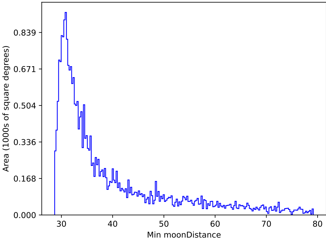
weather_cloudso20v3.4_10yrs All sky r band: Min moonDistance
