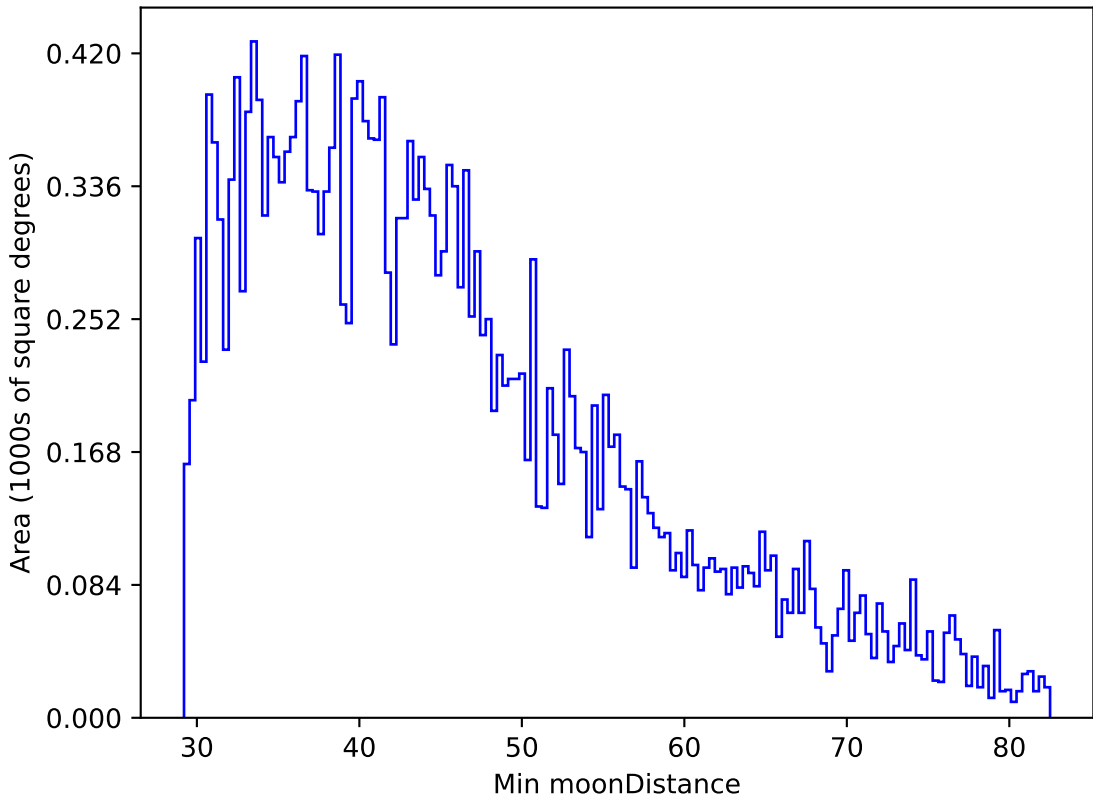
weather_cloudso20v3.4_10yrs All sky g band: Min moonDistance
