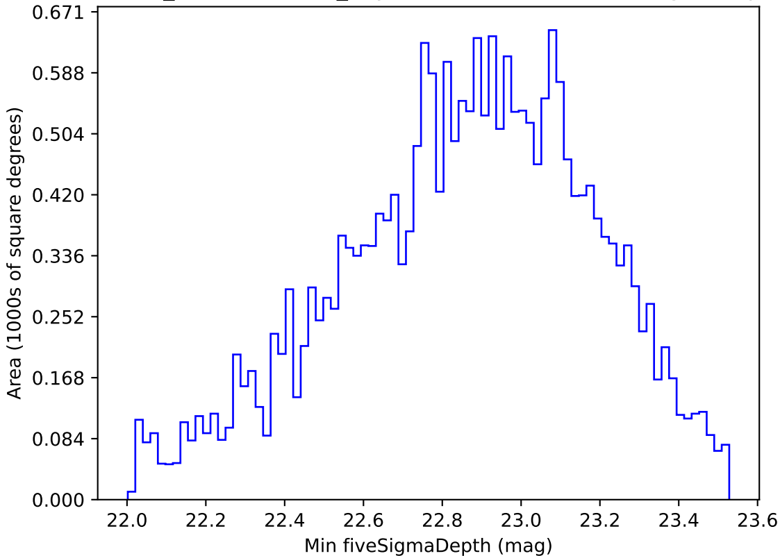
weather_cloudso20v3.4_10yrs Yr 1 u band: Min fiveSigmaDepth
