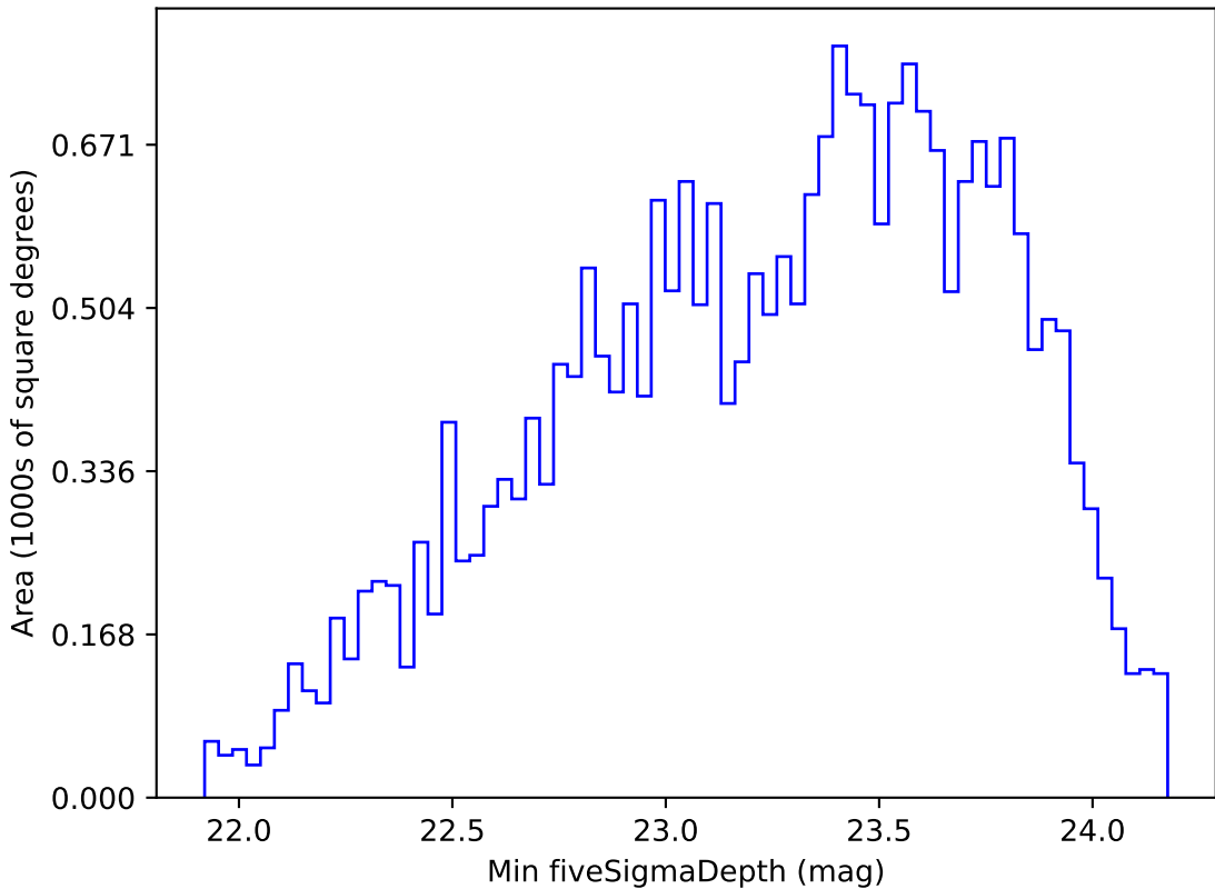
weather_cloudso20v3.4_10yrs Yr 1 r band: Min fiveSigmaDepth
