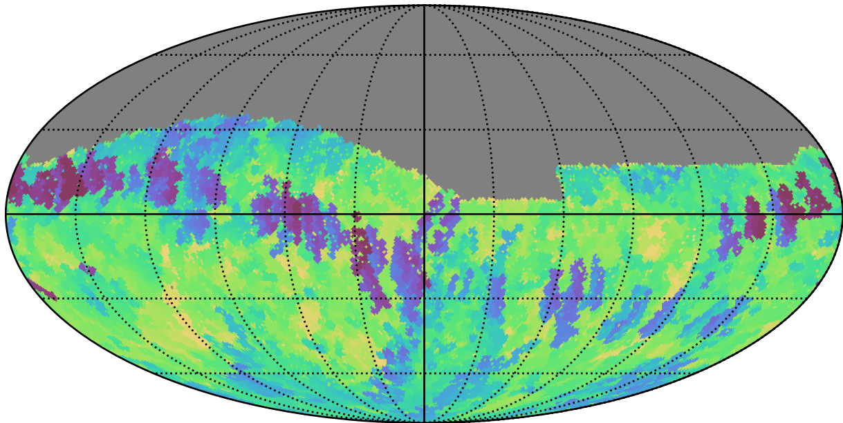
weather_cloudso20v3.4_10yrs Yr 1 i band: Min fiveSigmaDepth
