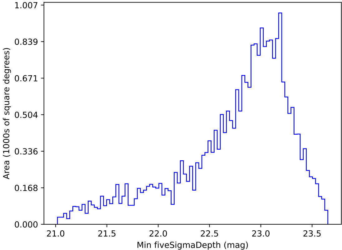
weather_cloudso20v3.4_10yrs Yr 1 i band: Min fiveSigmaDepth
