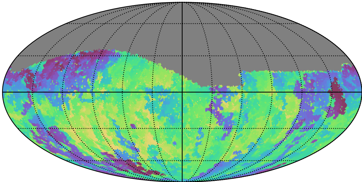
weather_cloudso20v3.4_10yrs Yr 1 g band: Min fiveSigmaDepth
