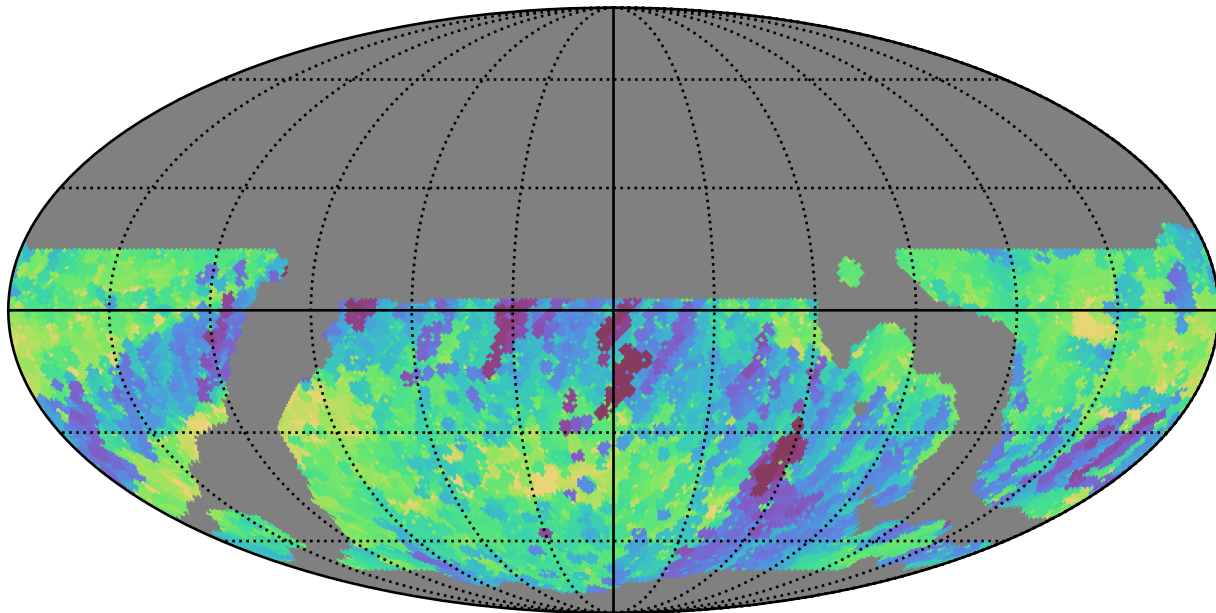
weather_cloudso20v3.4_10yrs WFD r band: Min fiveSigmaDepth
