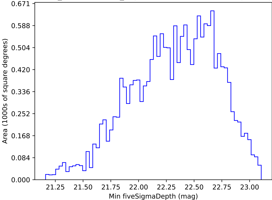
weather_cloudso20v3.4_10yrs WFD r band: Min fiveSigmaDepth
