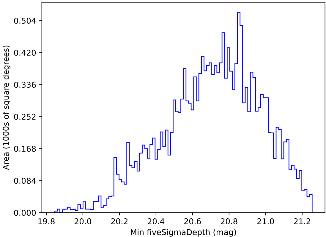
weather_cloudso20v3.4_10yrs WFD all bands: Min fiveSigmaDepth
