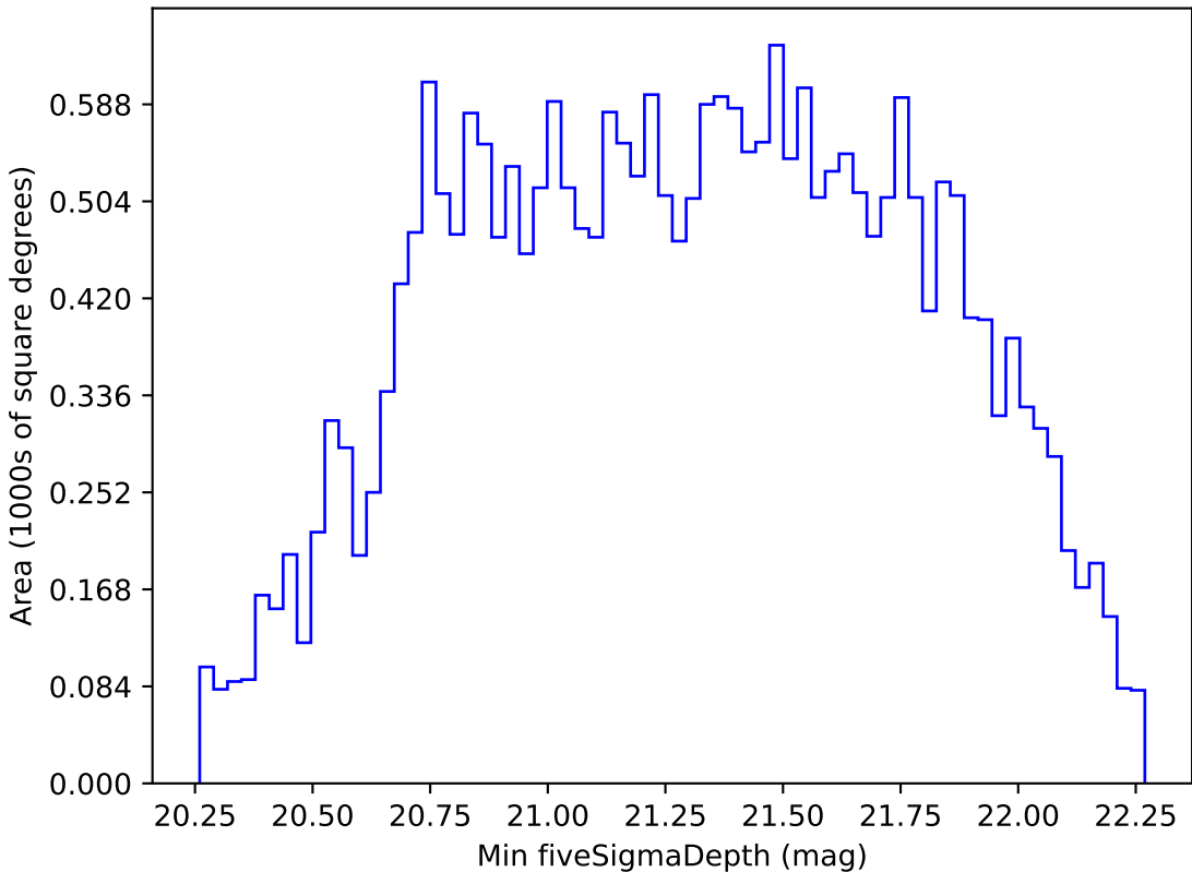
weather_cloudso20v3.4_10yrs All sky z band: Min fiveSigmaDepth
