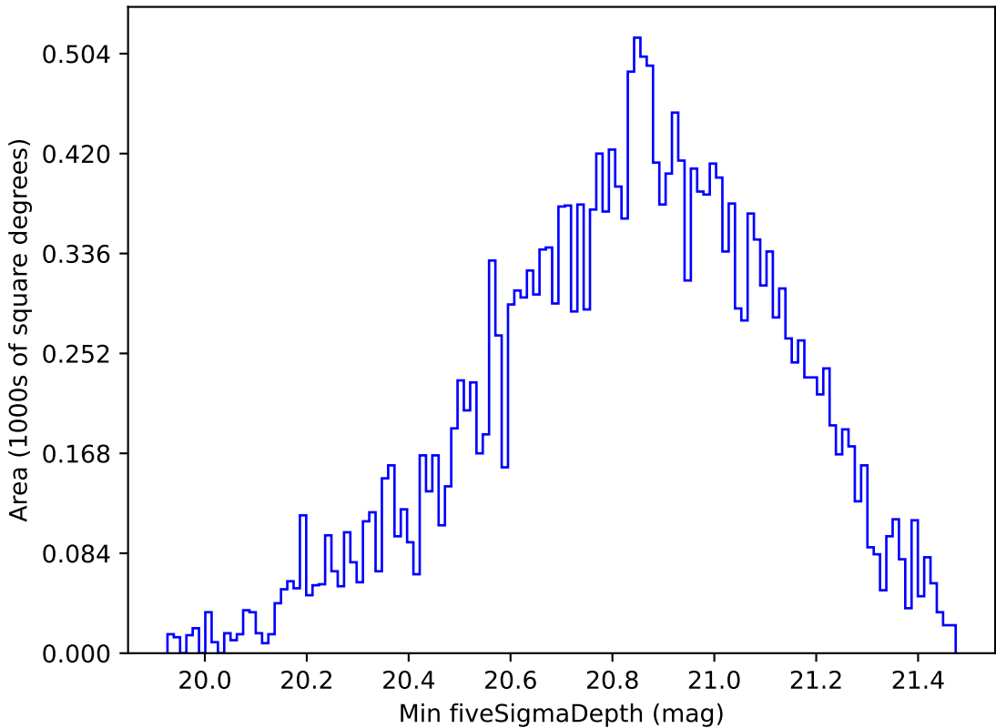
weather_cloudso20v3.4_10yrs All sky y band: Min fiveSigmaDepth
