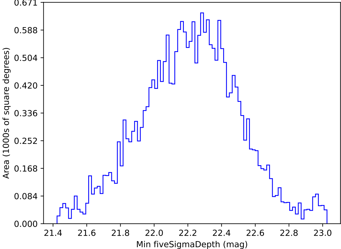
weather_cloudso20v3.4_10yrs All sky u band: Min fiveSigmaDepth
