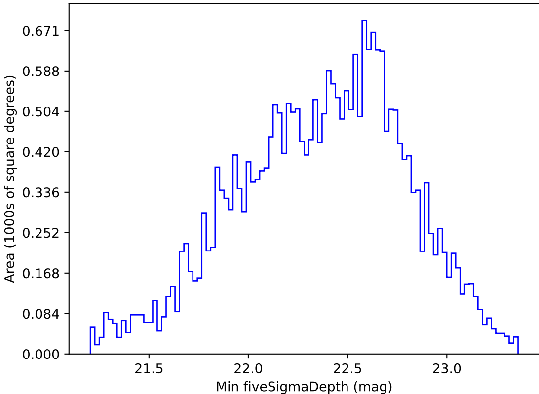
weather_cloudso20v3.4_10yrs All sky r band: Min fiveSigmaDepth
