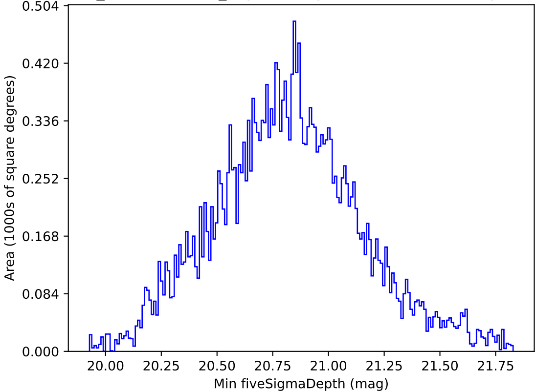
weather_cloudso20v3.4_10yrs All sky all bands: Min fiveSigmaDepth
