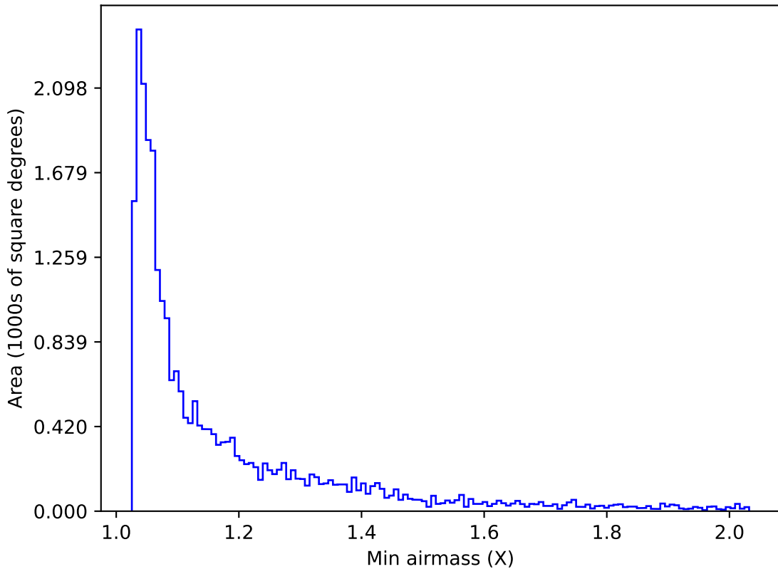
weather_cloudso20v3.4_10yrs Yr 1 z band: Min airmass
