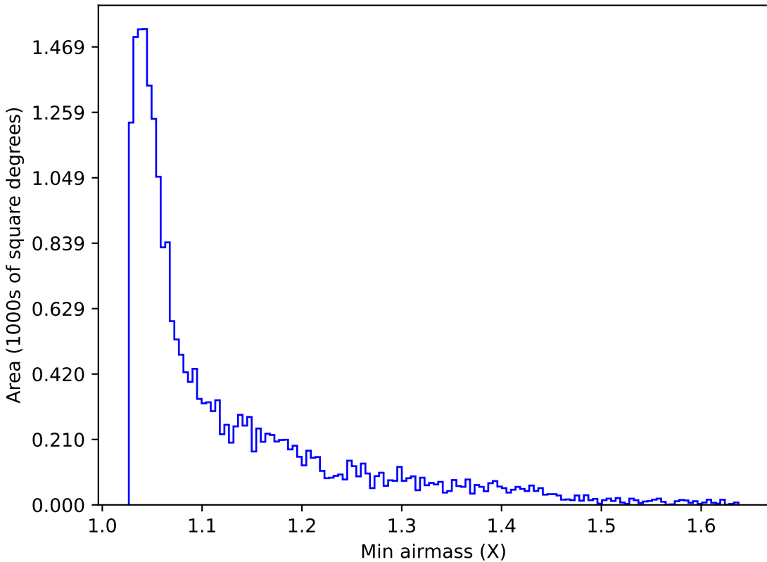
weather_cloudso20v3.4_10yrs Yr 1 y band: Min airmass
