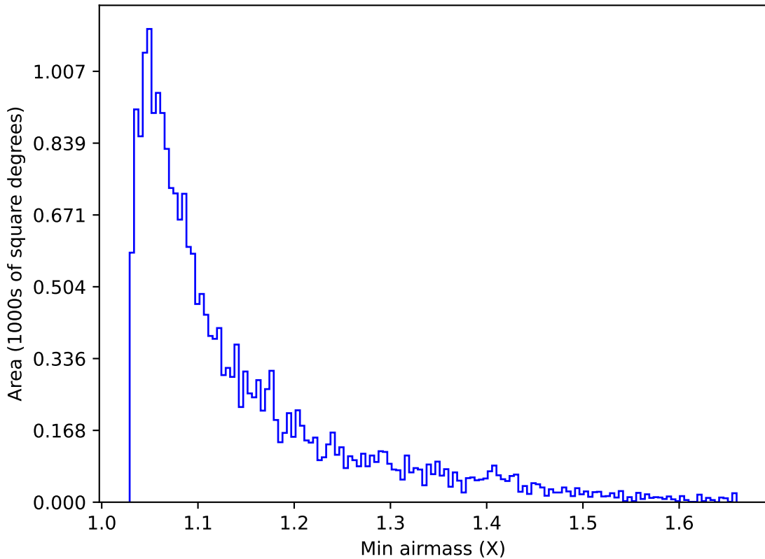
weather_cloudso20v3.4_10yrs Yr 1 u band: Min airmass
