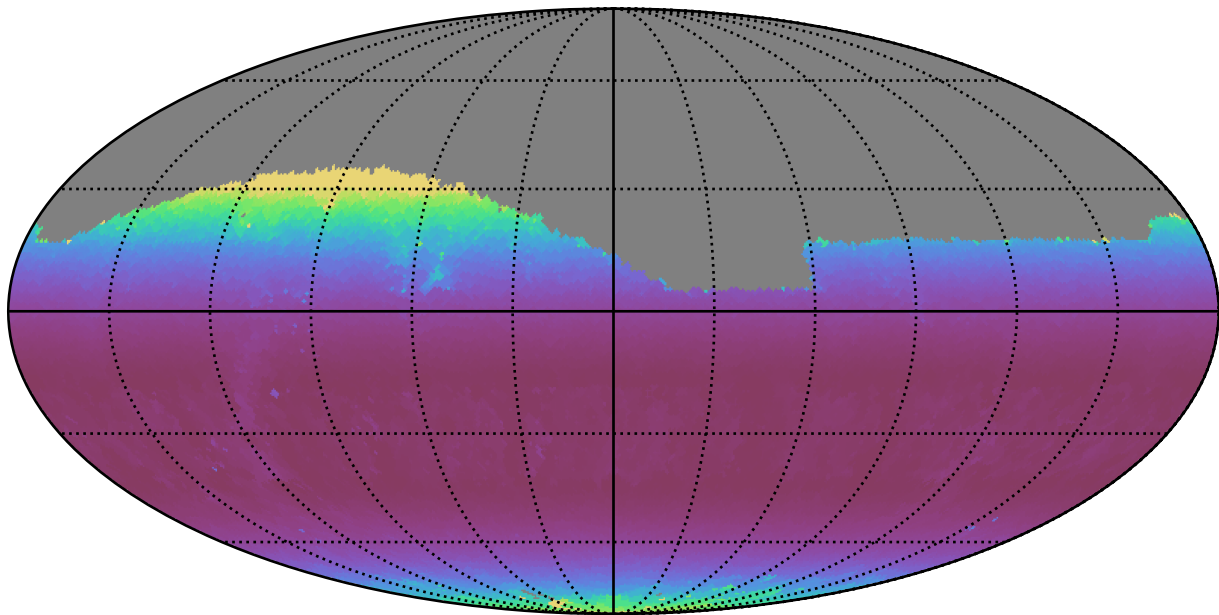
weather_cloudso20v3.4_10yrs Yr 1 r band: Min airmass
