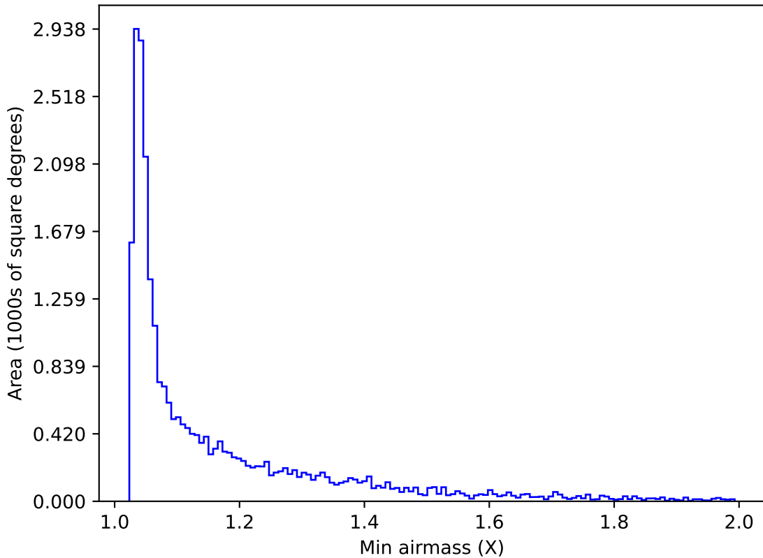
weather_cloudso20v3.4_10yrs Yr 1 r band: Min airmass
