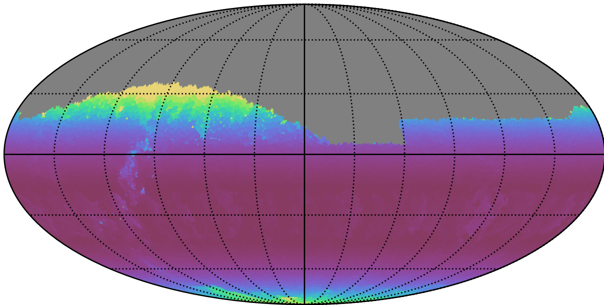
weather_cloudso20v3.4_10yrs Yr 1 i band: Min airmass
