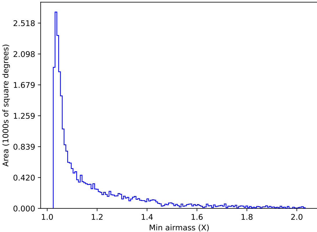
weather_cloudso20v3.4_10yrs Yr 1 i band: Min airmass
