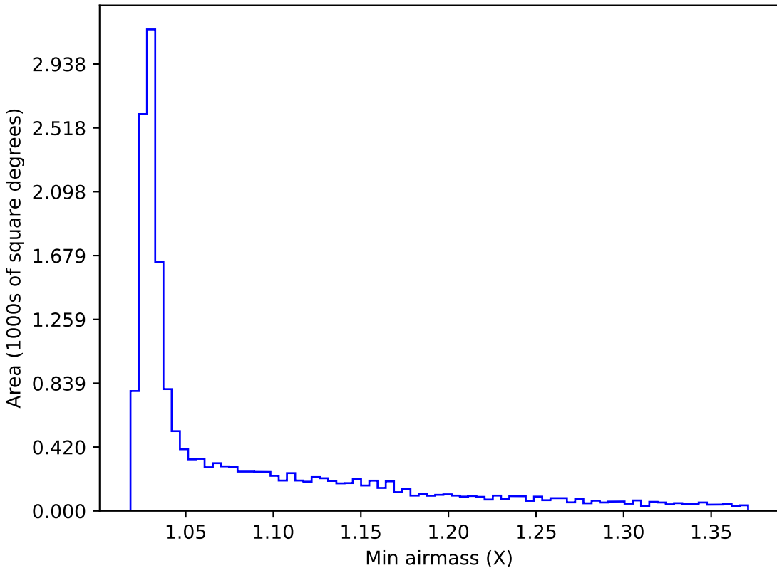
weather_cloudso20v3.4_10yrs WFD z band: Min airmass
