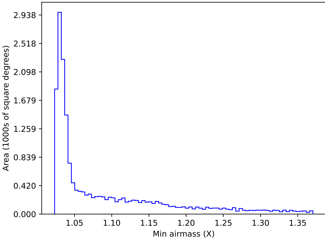
weather_cloudso20v3.4_10yrs WFD y band: Min airmass
