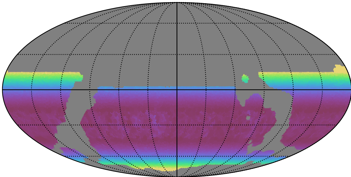
weather_cloudso20v3.4_10yrs WFD u band: Min airmass
