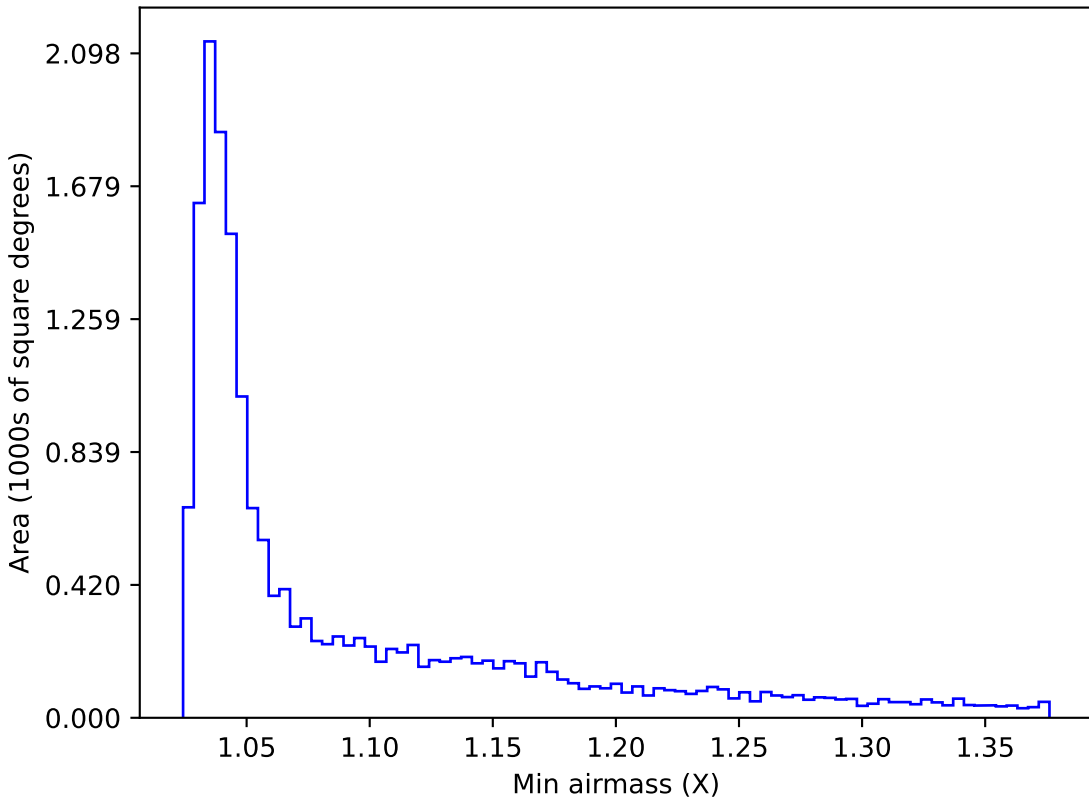
weather_cloudso20v3.4_10yrs WFD u band: Min airmass
