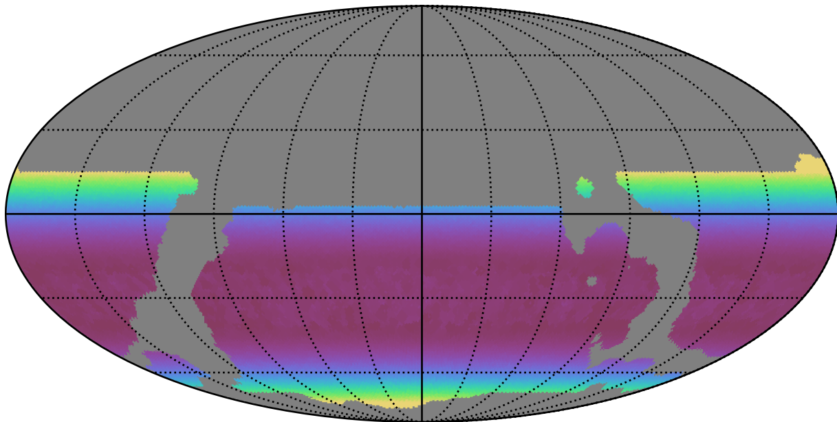
weather_cloudso20v3.4_10yrs WFD r band: Min airmass
