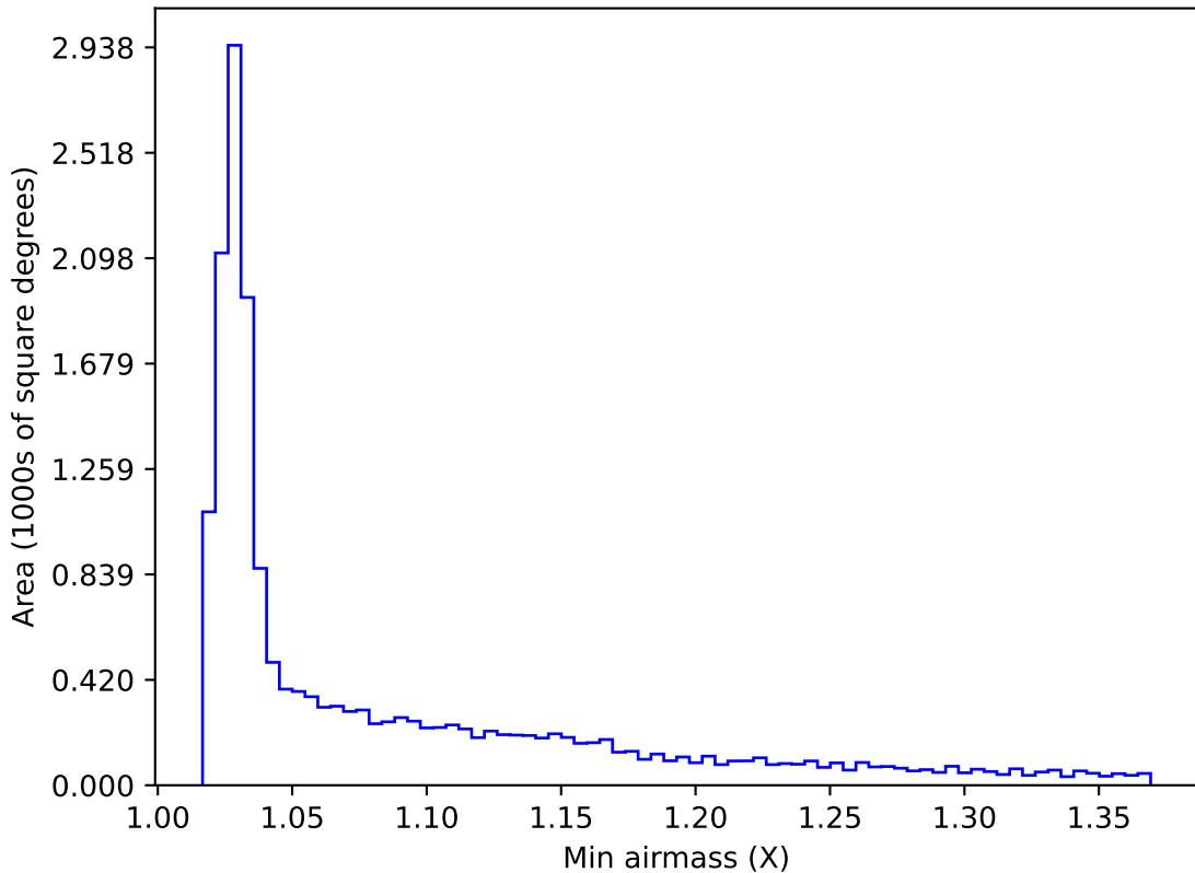
weather_cloudso20v3.4_10yrs WFD r band: Min airmass
