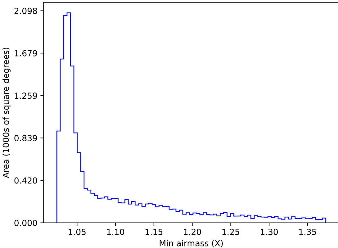
weather_cloudso20v3.4_10yrs WFD g band: Min airmass
