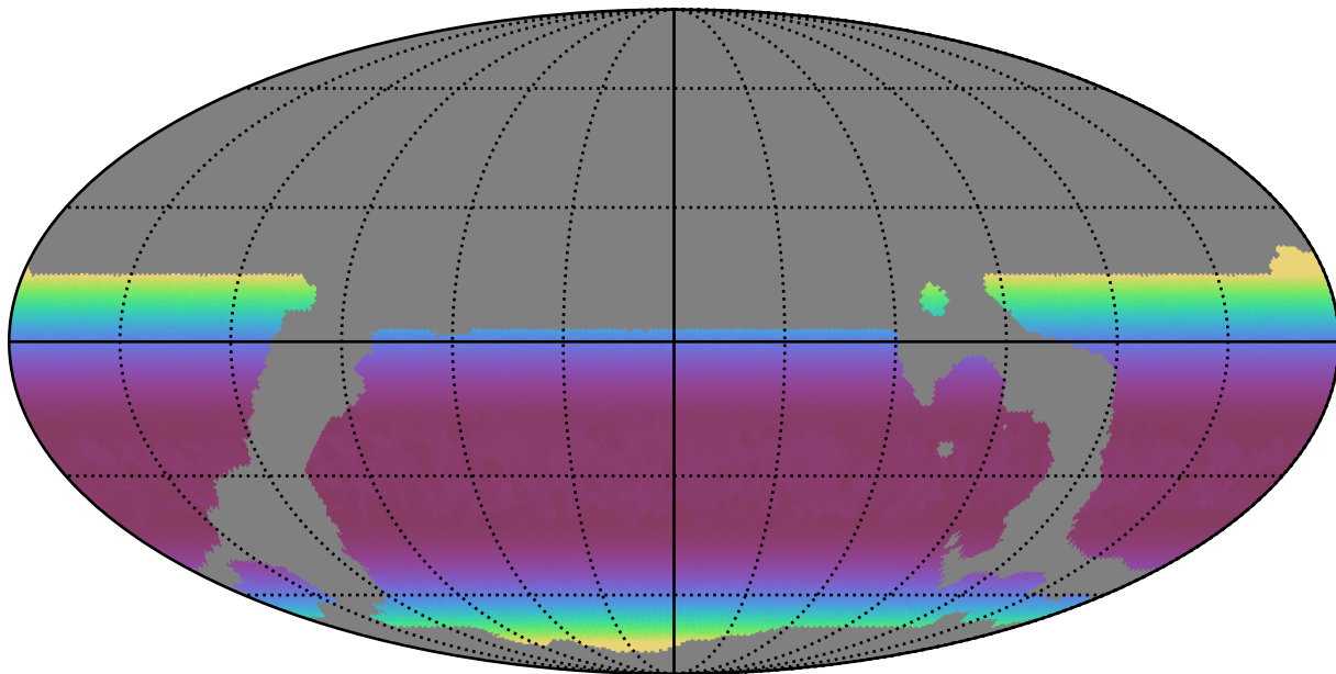
weather_cloudso20v3.4_10yrs WFD all bands: Min airmass
