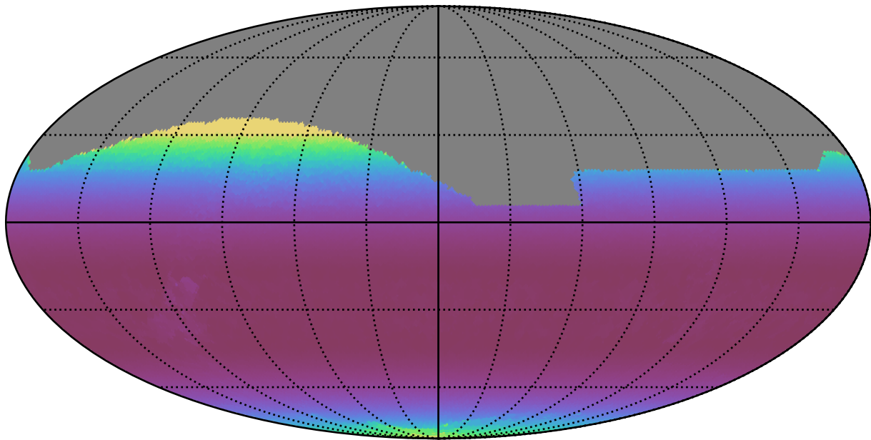
weather_cloudso20v3.4_10yrs All sky z band: Min airmass
