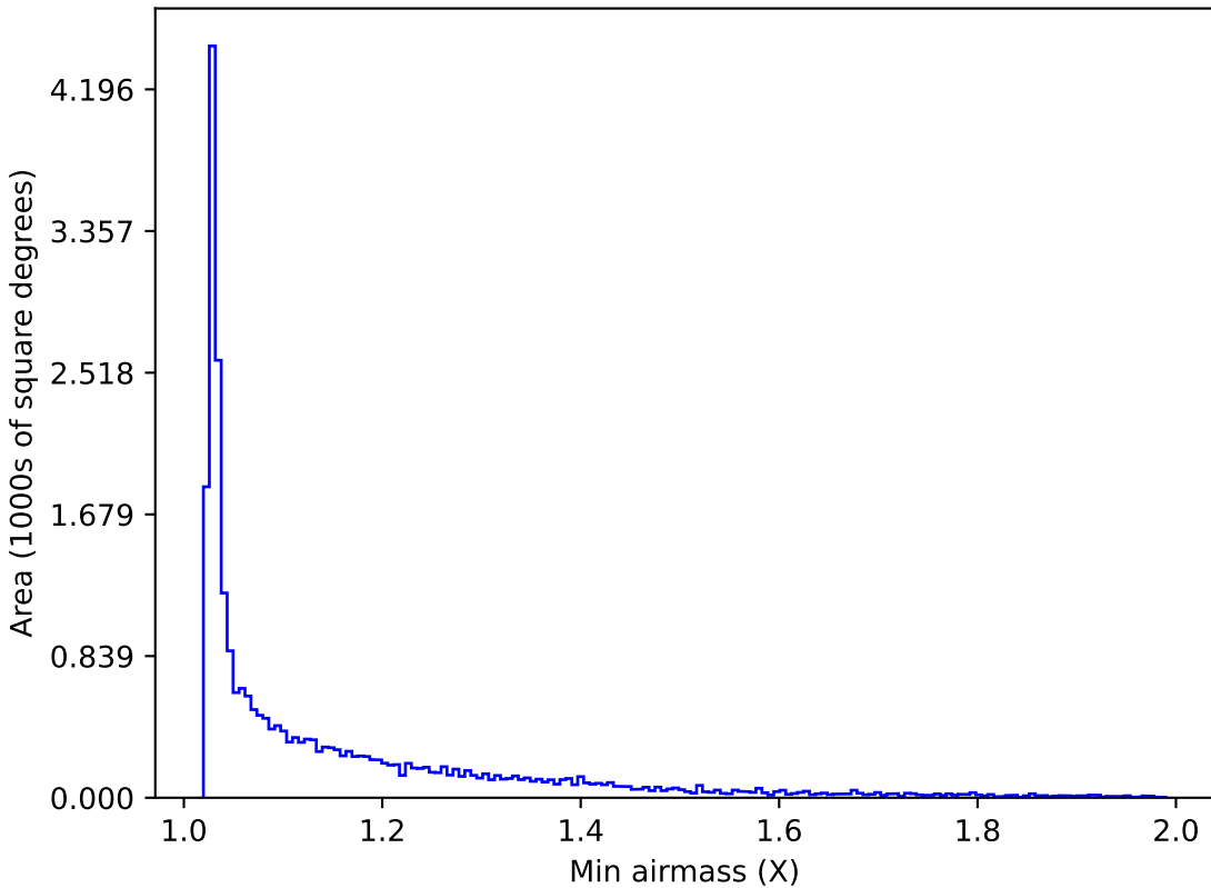
weather_cloudso20v3.4_10yrs All sky z band: Min airmass
