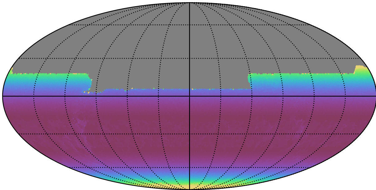
weather_cloudso20v3.4_10yrs All sky y band: Min airmass
