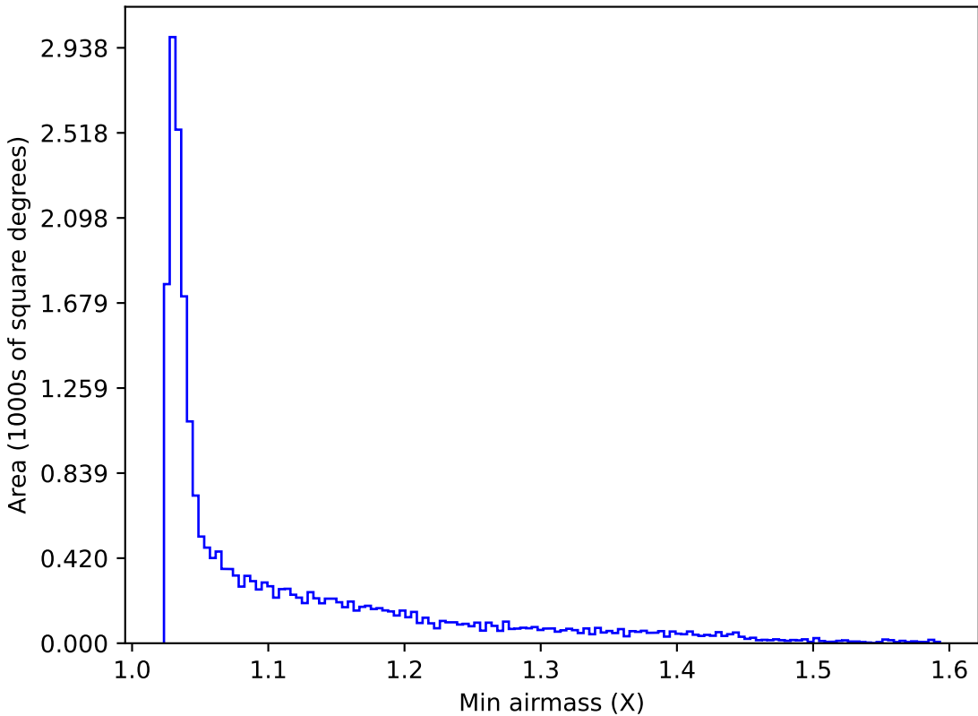
weather_cloudso20v3.4_10yrs All sky y band: Min airmass
