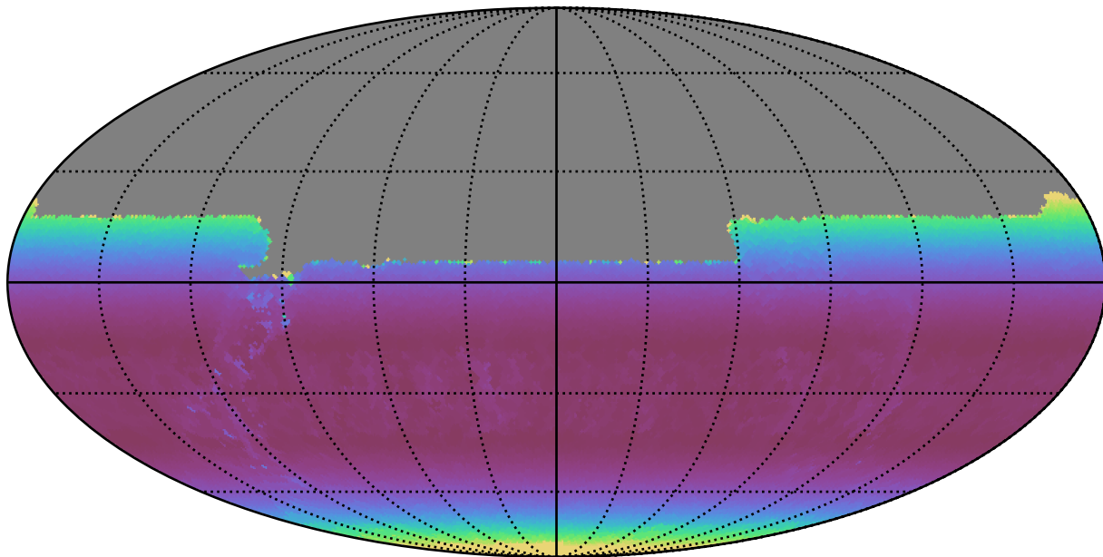
weather_cloudso20v3.4_10yrs All sky u band: Min airmass
