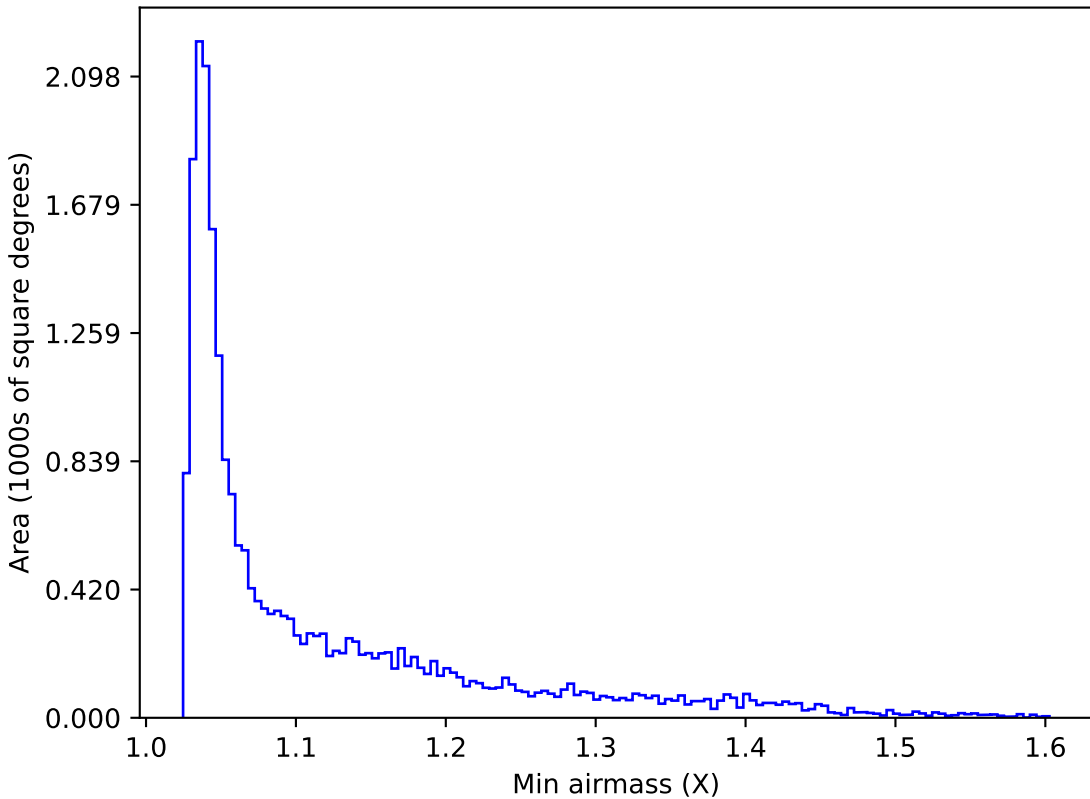
weather_cloudso20v3.4_10yrs All sky u band: Min airmass
