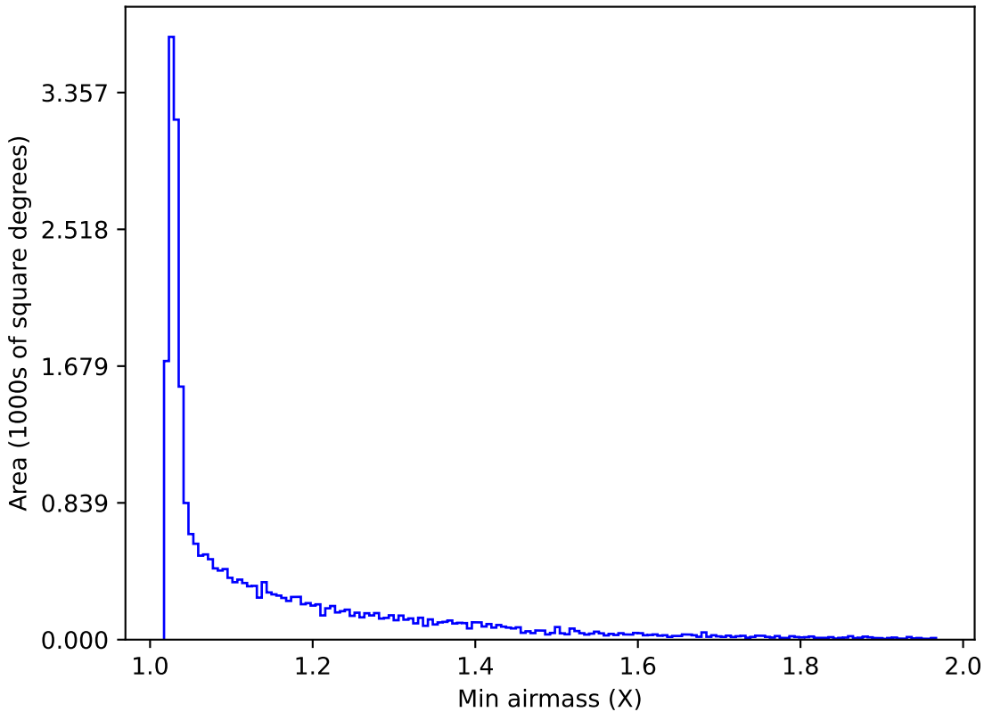
weather_cloudso20v3.4_10yrs All sky r band: Min airmass
