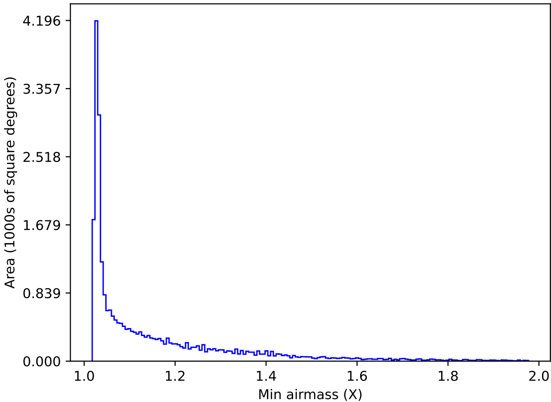
weather_cloudso20v3.4_10yrs All sky i band: Min airmass
