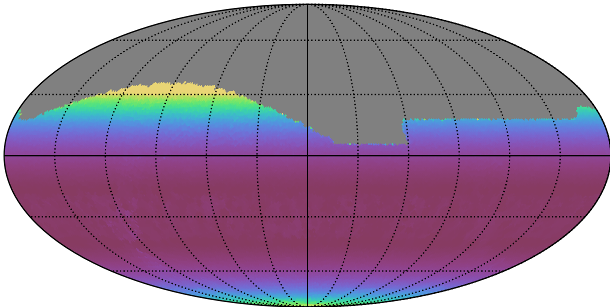
weather_cloudso20v3.4_10yrs All sky g band: Min airmass
