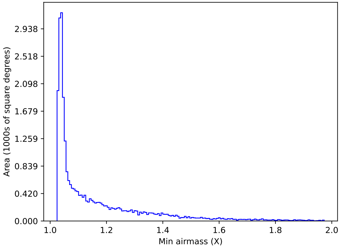
weather_cloudso20v3.4_10yrs All sky g band: Min airmass
