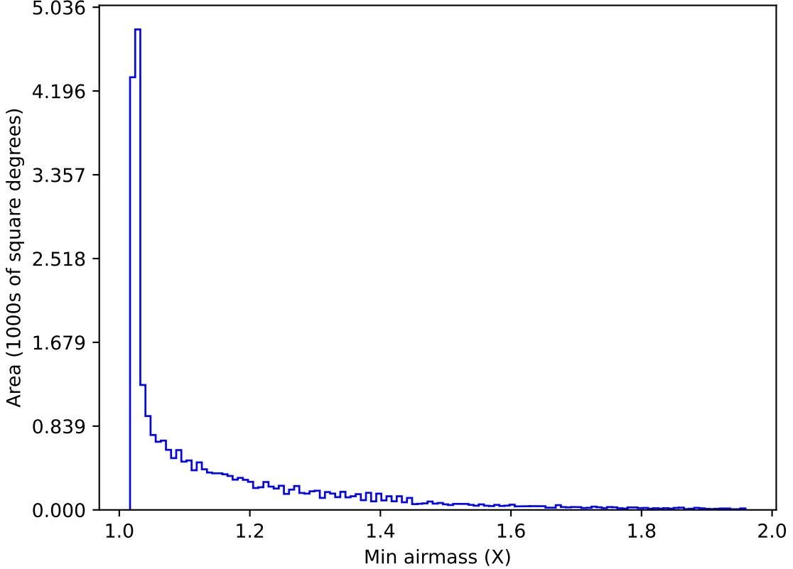
weather_cloudso20v3.4_10yrs All sky all bands: Min airmass
