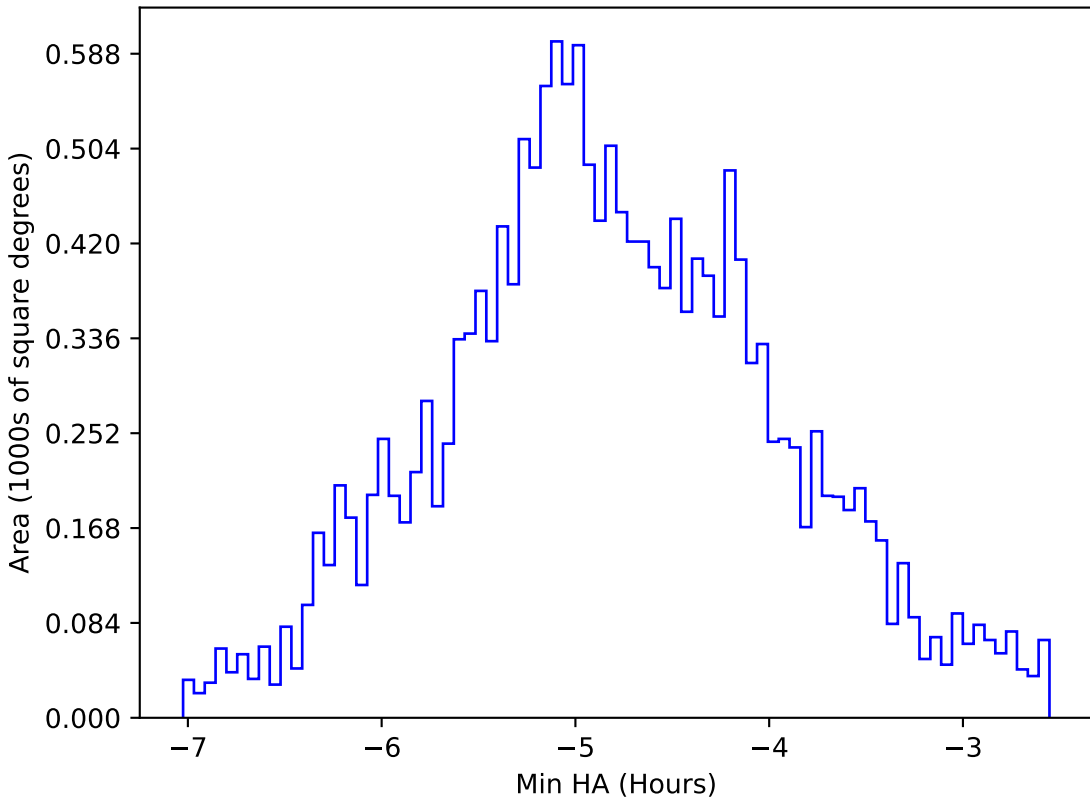
weather_cloudso20v3.4_10yrs WFD all bands: Min HA
