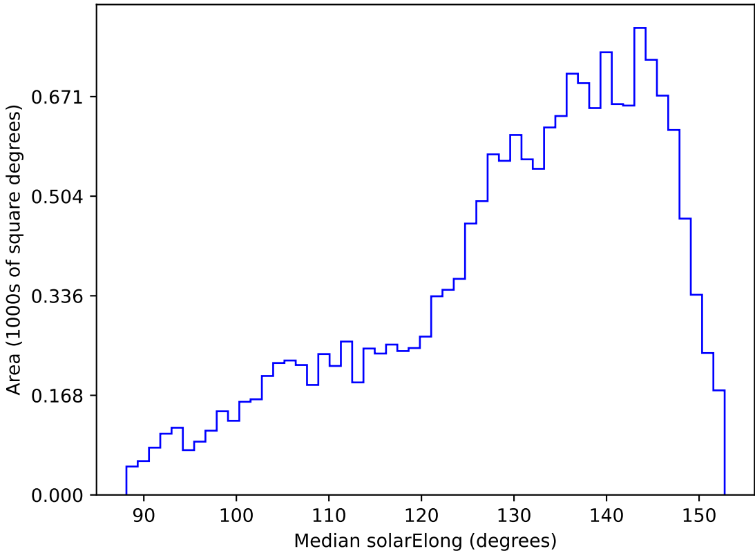
weather_cloudso20v3.4_10yrs WFD u band: Median solarElong
