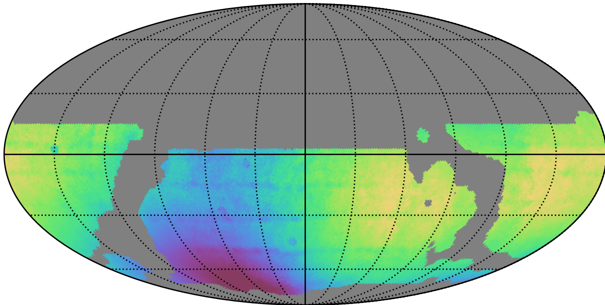
weather_cloudso20v3.4_10yrs WFD all bands: Median solarElong
