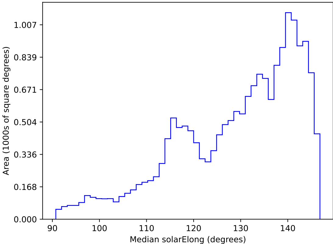
weather_cloudso20v3.4_10yrs WFD all bands: Median solarElong
