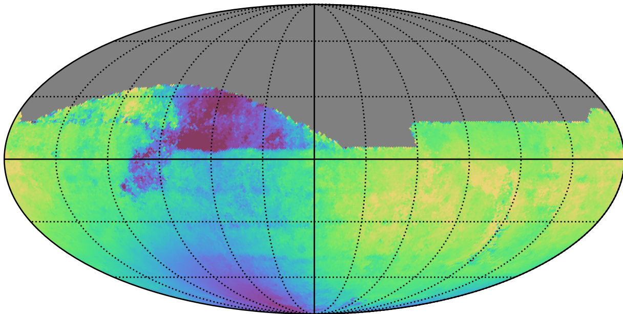
weather_cloudso20v3.4_10yrs All sky z band: Median solarElong
