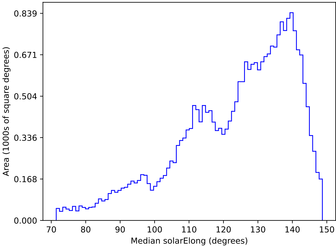
weather_cloudso20v3.4_10yrs All sky z band: Median solarElong
