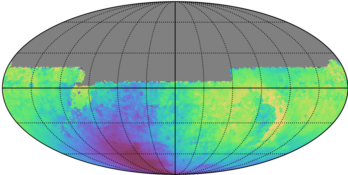
weather_cloudso20v3.4_10yrs All sky u band: Median solarElong
