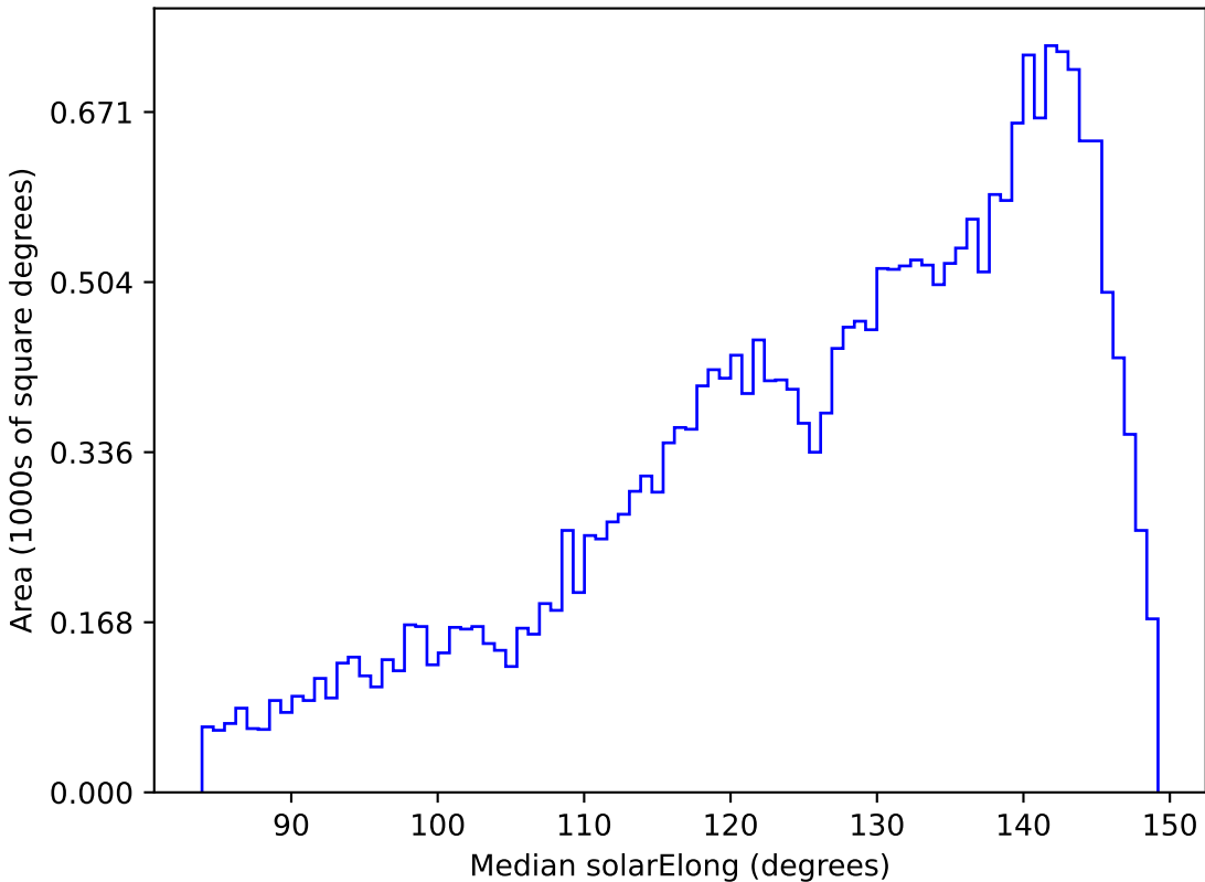
weather_cloudso20v3.4_10yrs All sky r band: Median solarElong
